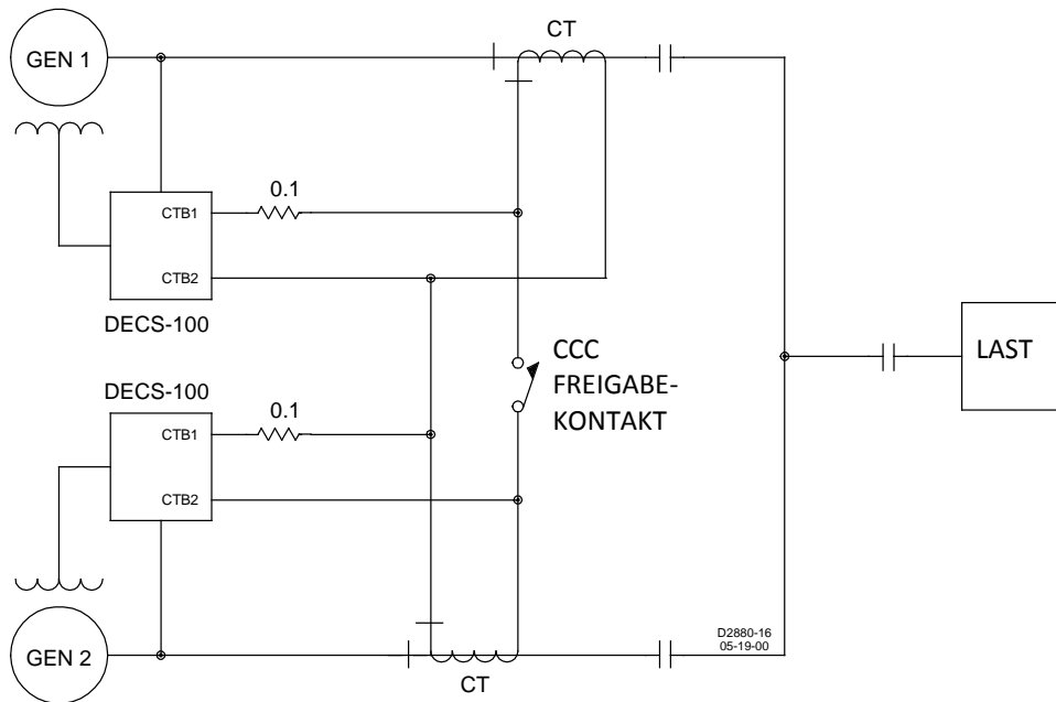
Abbildung 4-11. Querstromanschlüsse (induktives Differential)
