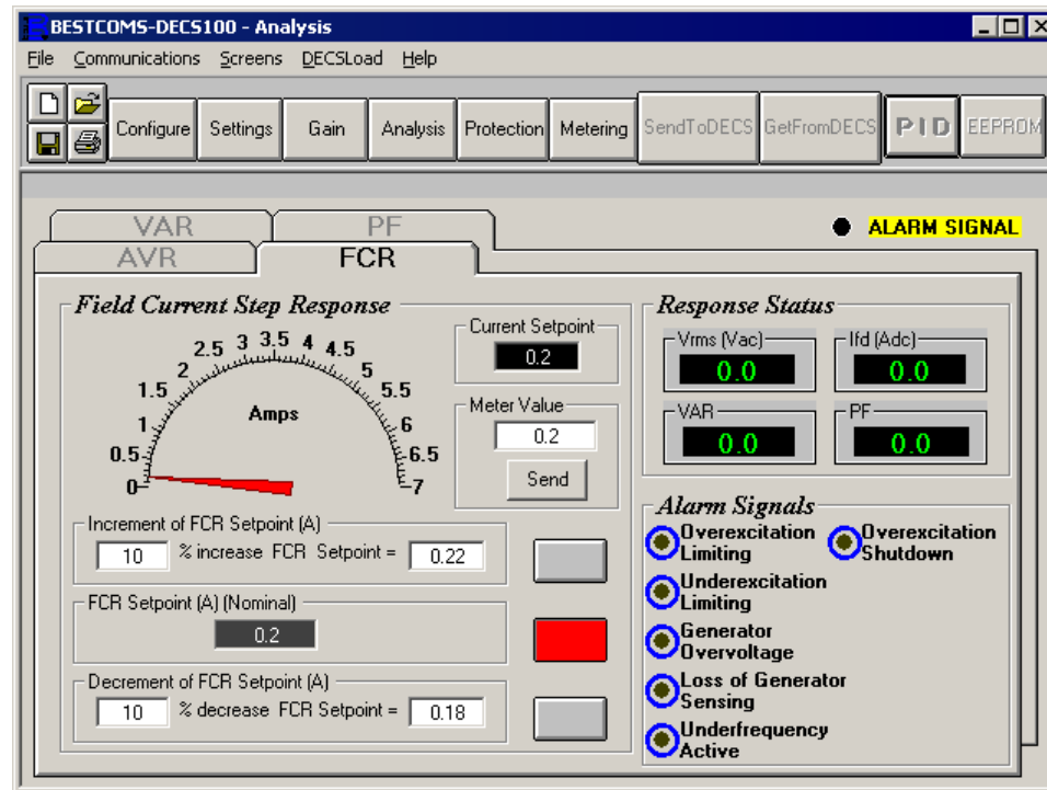
Figure 5-11. Ecran analyse, onolet FCR
