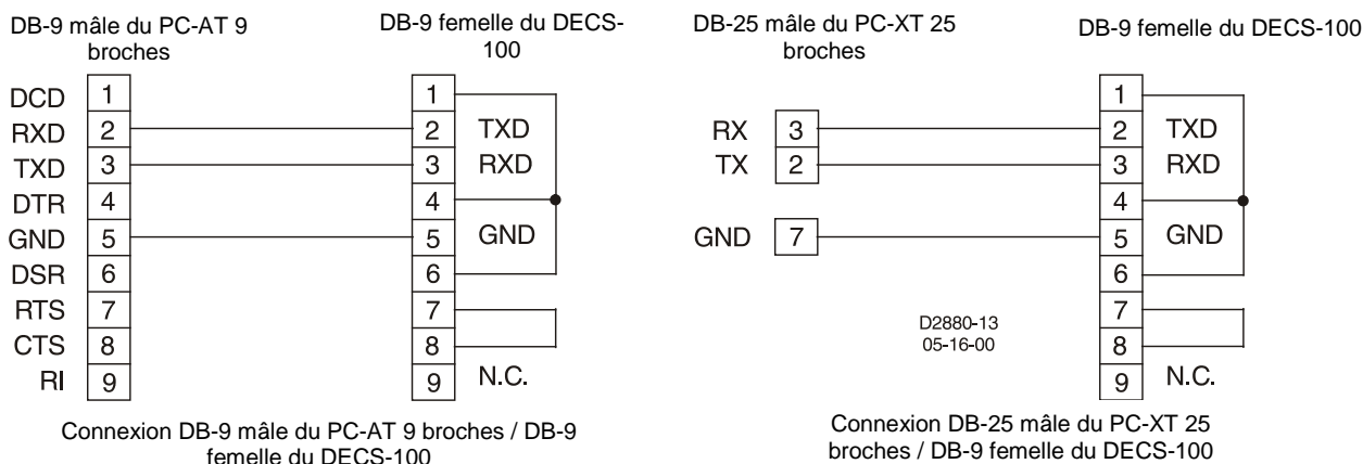
Figure 4-5. Connexions PC/DECS-100
