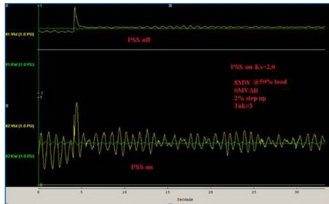
Figure 6b - 2% voltage step change demonstrating poor response from the Lead/Lag filter tuning in Figure 6a
