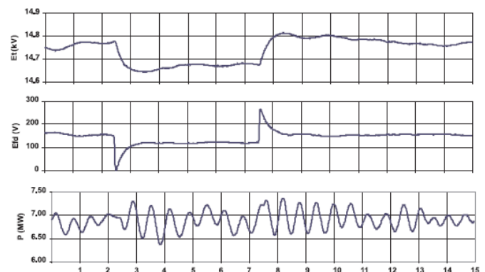
Figure 2 - Power system oscillations following a unit disturbance
