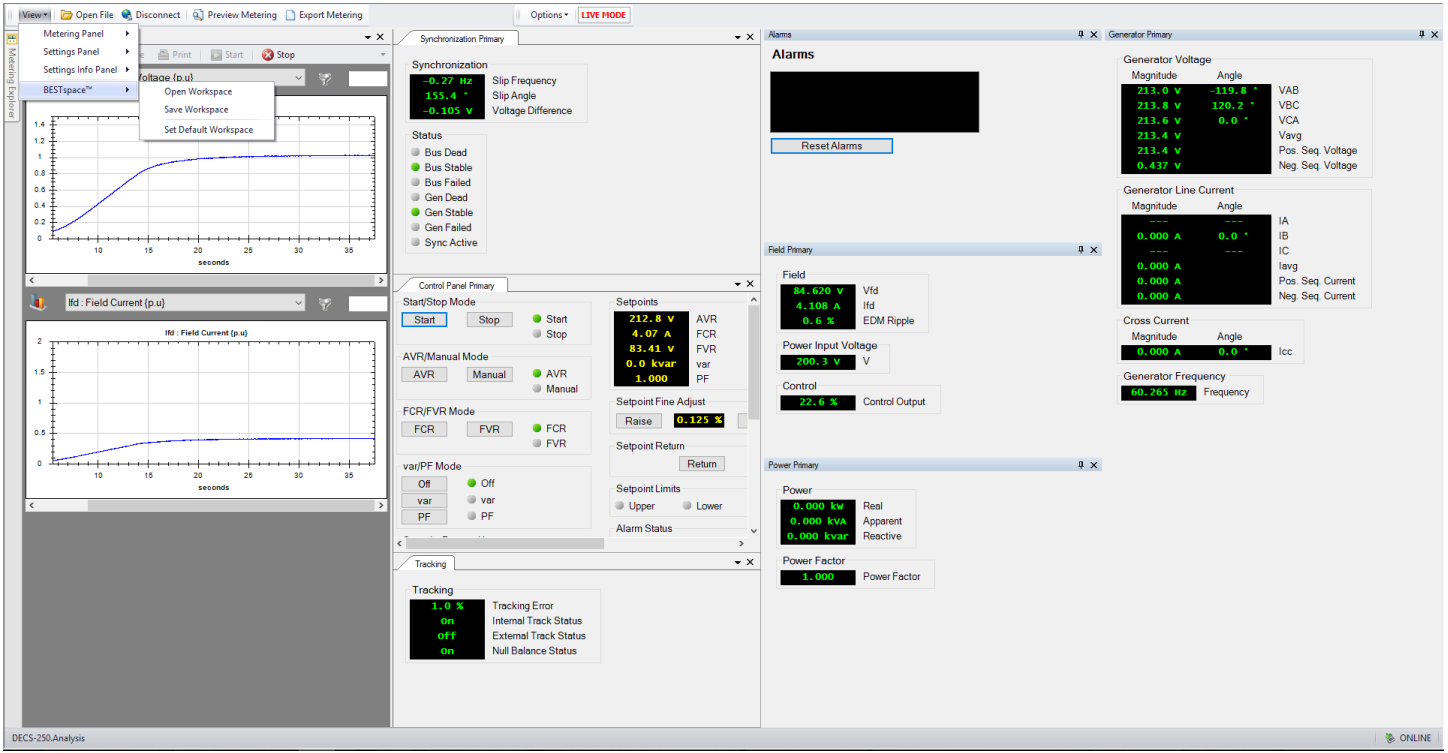
Figure 10: BESTspace
